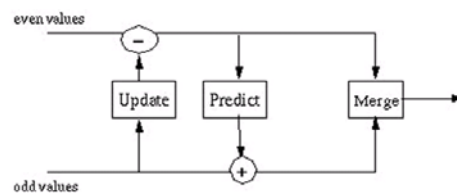
Fig. 9. Lifting scheme inverse wavelet transformation
