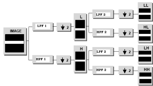
Fig. 7. One-level decomposition using the two-dimensional DWT, where LPF1 Represents low-pass filtering of the image rows, HPF1 represents high-pass filtering of Image rows, LPF2 represents low-pass filtering of image columns, and HPF2 represents high-pass filtering of image columns.
