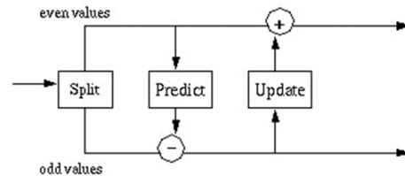
Fig. 8. Lifting scheme forward wavelet transformation
