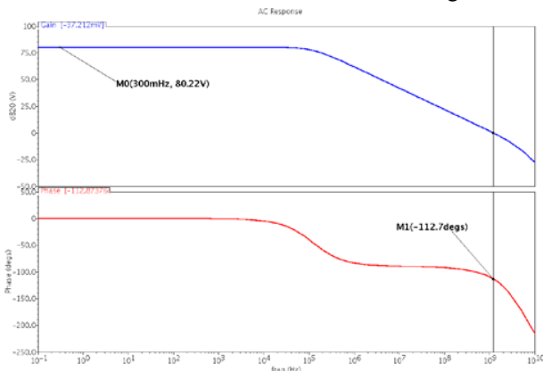
Fig. 9 AC response
