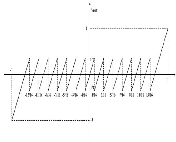
Fig. 2 The transfer function of 3.5-bit stage
