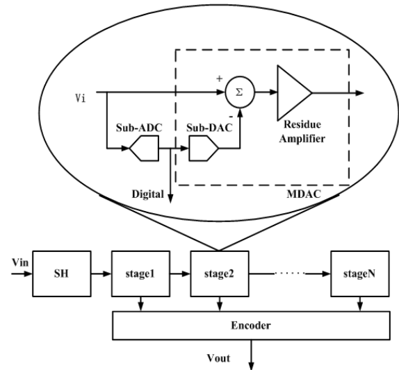
Fig. 1 General pipelined ADC architecture
