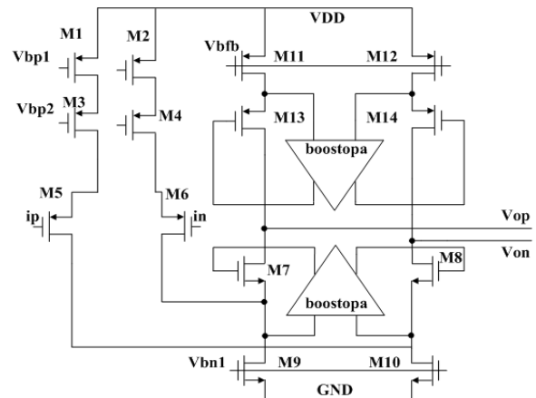
Fig. 6 The main form of the amplifier
