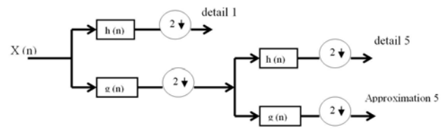
Fig. 1. Decomposed levels of DWT
