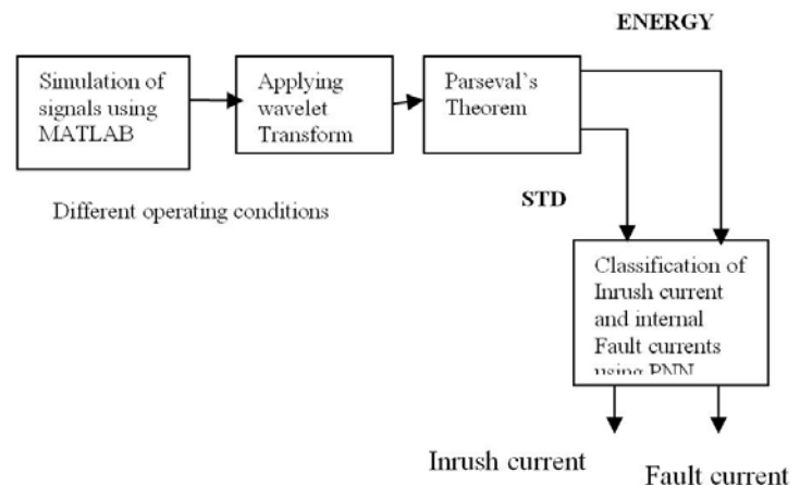
Fig. 3. Block diagram for the proposed
