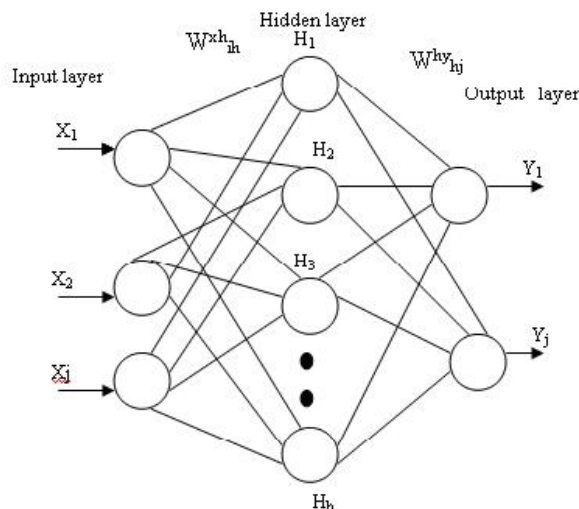
Fig. 7. PNN architecture for transformer fault
