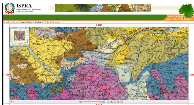
Fig. 5 Geological map - supplied by ISPRA
