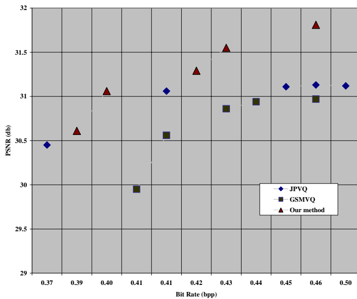
Fig. 5 Experimental results in terms of PSNR and bit rate for JPVQ, GSMVQ and our method with Jet as the standard test image
