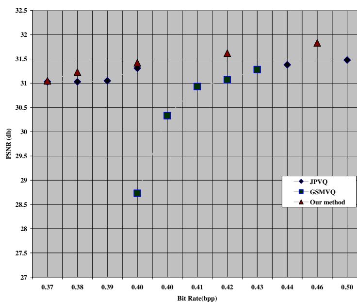
Fig. 6 Experimental results in terms of PSNR and bit rate for JPVQ, GSMVQ and our method with Pepper as the standard test image
