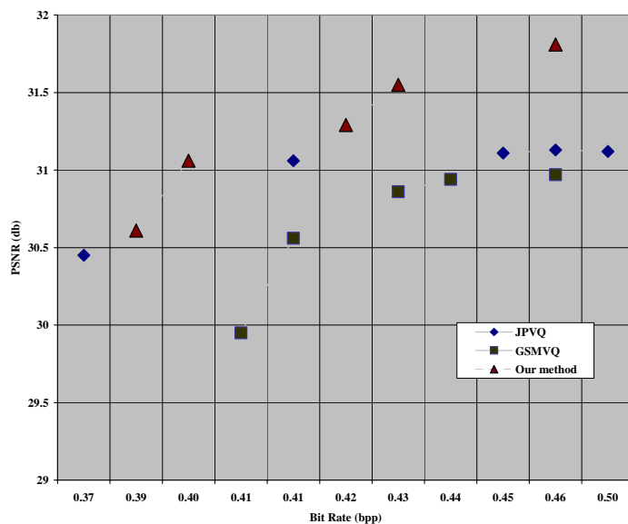
Fig. 4 Experimental results in terms of PSNR and bit rate for JPVQ, GSMVQ and our method with Lena image as the standard test image
