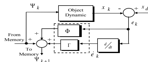
Fig.3 PD type learning algorithm
