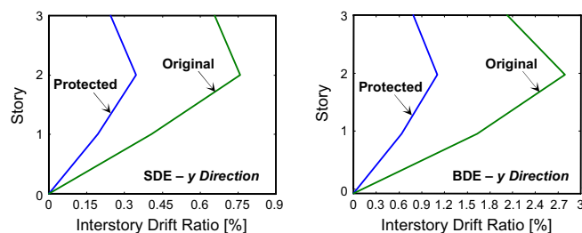
Fig. 6 Maximum interstory drift profiles in y direction (mean values)
