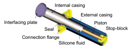
Fig. 2 Perspective cross section of a pressurized FV spring-damper
