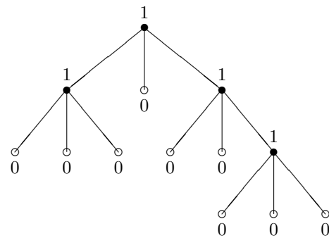
Fig. 1. A 3-ary tree with 4 internal nodes.
