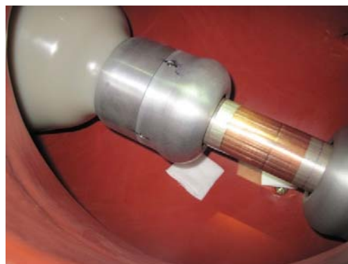
Fig. 3 The conductive rod in GIS tank
