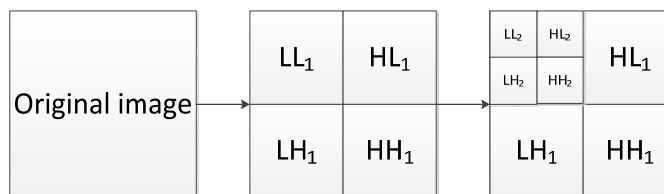
Fig. 2 wavelet decomposition
