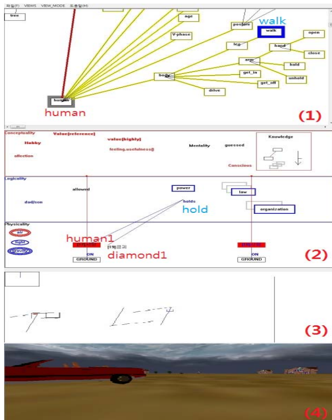
Fig. 4 The main screen of S-T graph system
