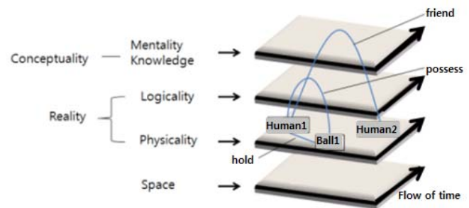
Fig. 2 The structure of S-T graph
