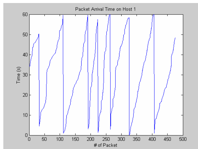
Fig. 4 Packet Arrival Time for Host 1
