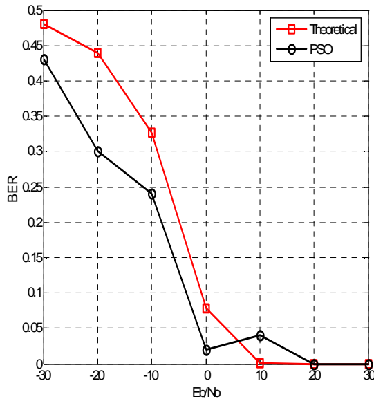
Fig. 4 Theoretical and PSO Comparison of BER
