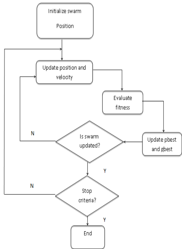
Fig. 2 PSO Flowchart
