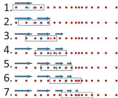
Fig. 7. Mean Shift Algorithm
