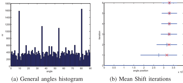
Fig. 9. Mean Shift Algorithm for angle computation
