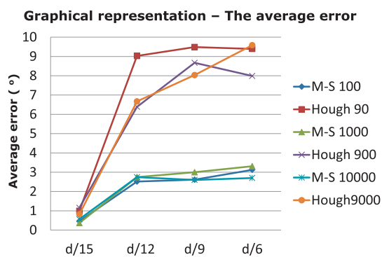
Fig. 19. The average error
