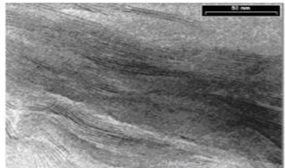
Fig. 2- The image of microscopic transient electron of epoxy nano composite 3 weight percent clay
