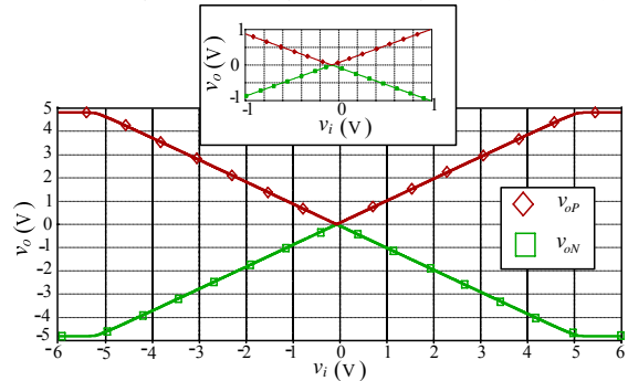
Fig. 5 DC transfer characteristic of the proposed positive/negative full-wave rectifier
