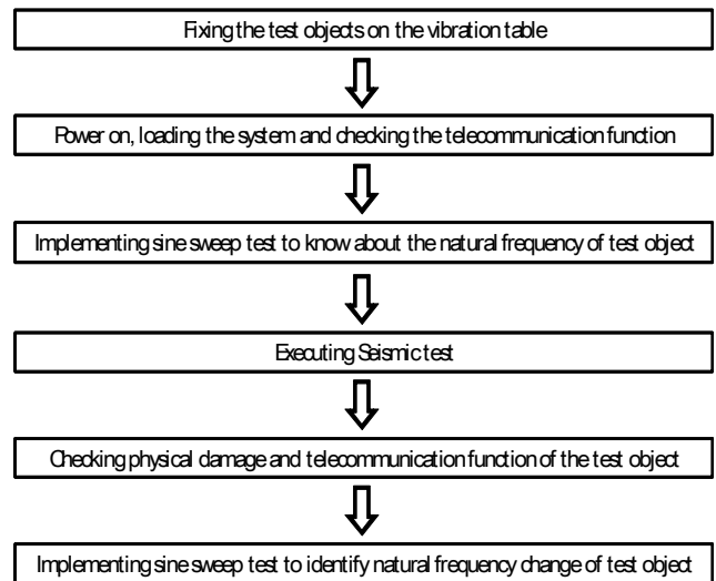
Fig. 1 The seismic test process of telecommunication equipments
