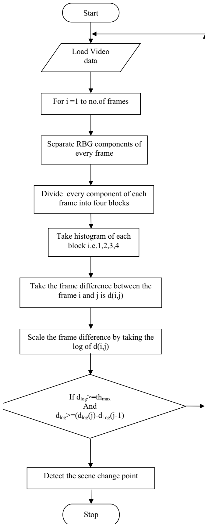
Fig. 2 Flow chart for abrupt change in video transition
