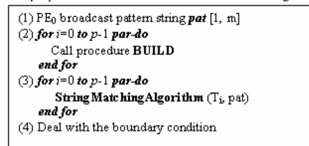
Fig. 1 The distributed string matching algorithm architecture
