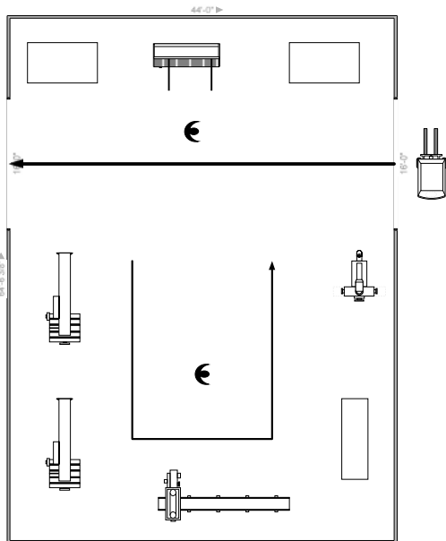
Fig. 4 Improved layout of woodworks area
