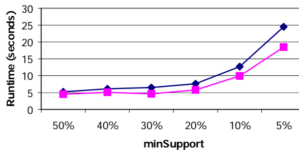
(b) Chess data
