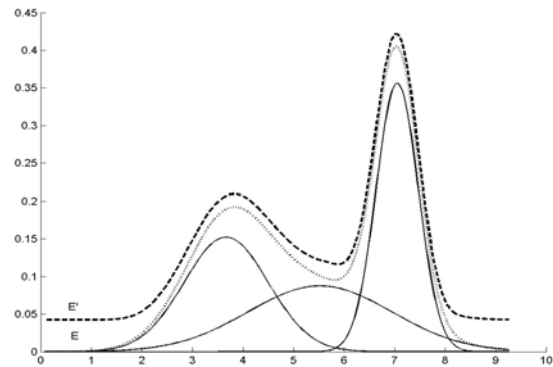
Fig. 1 Rejection sampling with an upper bound E'
