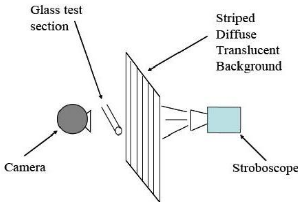
Fig. 3 Flow visualization schematic
