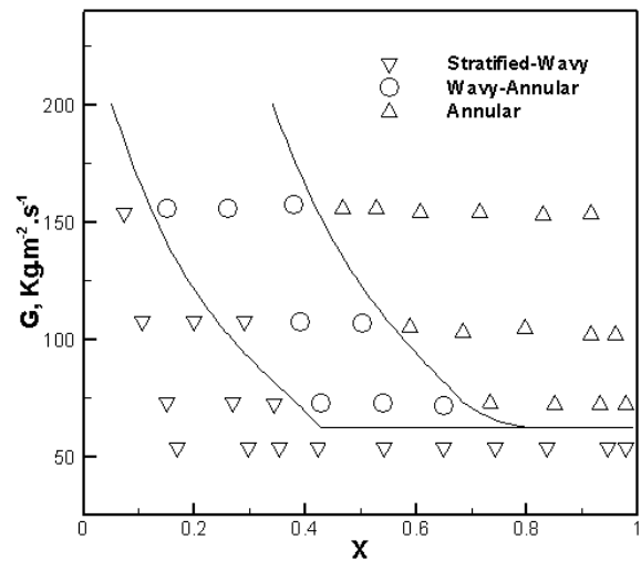
Fig. 8 G - x flow pattern map for horizontal smooth tube
