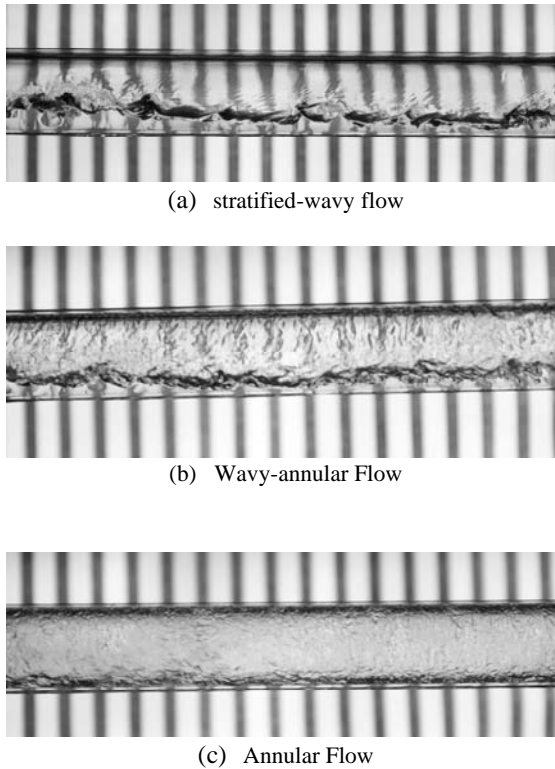
Fig. 4 Flow patterns in horizontal microfin and plain tube
