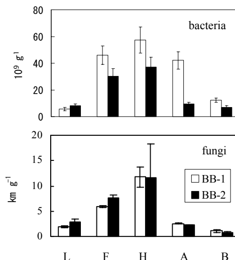
Fig. 4 The bacterial number and fungal hyphal length in laurel-leaved (BB-1) and C. japonica (BB-2) forest soils determined by the direct microscopic count method
