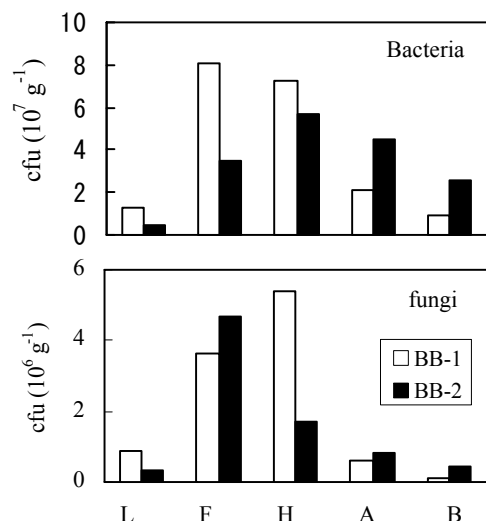
Fig. 3 The numbers of bacteria and fungi in laurel-leaved (BB-1) and C. japonica (BB-2) forest soils obtained by the dilution plate count method
