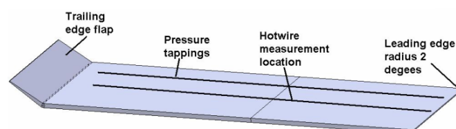
Fig. 1: Flat plate design features and measurement locations
