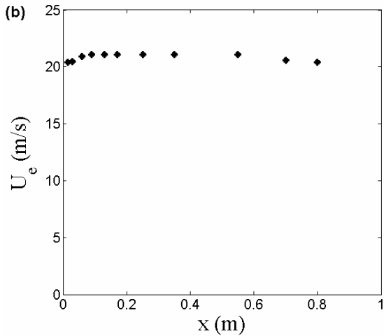
Fig. 7: (a) Mean velocity profiles over the plate compared to the Blasius profile. (b) Velocity distribution over the plate using (1).
