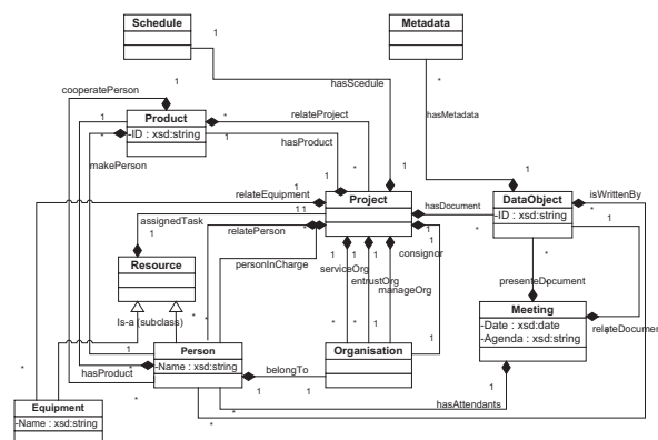
Fig. 4 Ontology Model
