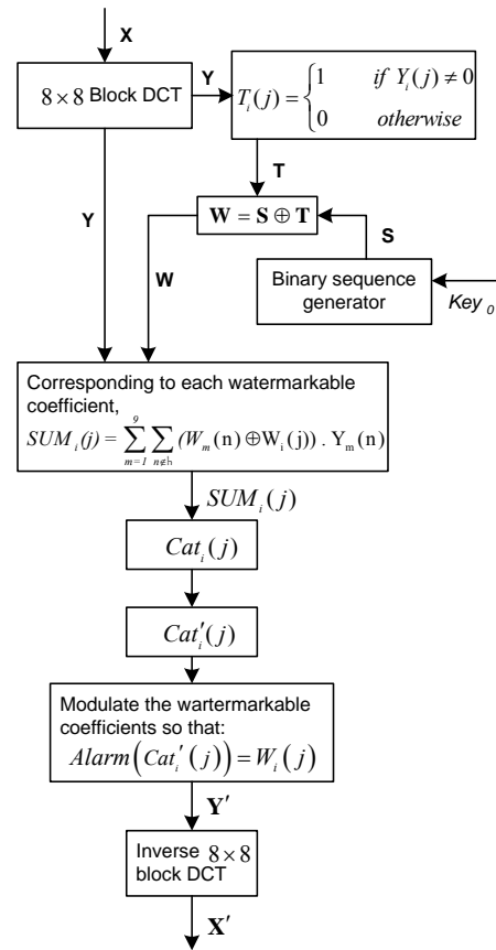
Fig. 2 Block diagram of the watermarking embedding algorithm
