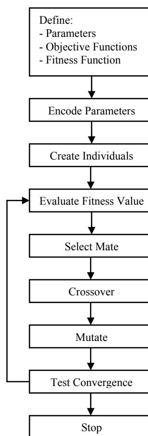
Fig. 1 The Flow chart of a typical Genetic Algorithm
