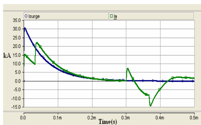
Fig. 17 Current waveform of lightning surge, I_{surge} (blue curve), current of the point hit by lightning in phase A, I_a (green curve)
