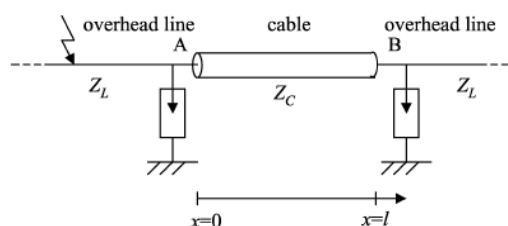
Fig. 13 Overhead line- Underground transition [7]
