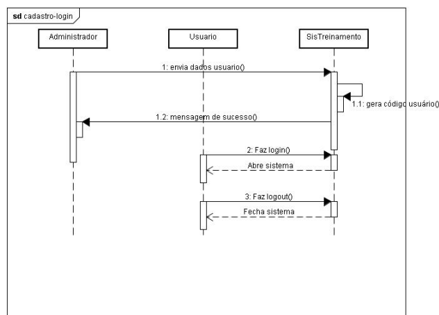
Fig. 5 Sequence diagram "Register and Login"
