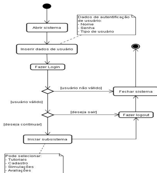
Fig. 4 Activity diagram
