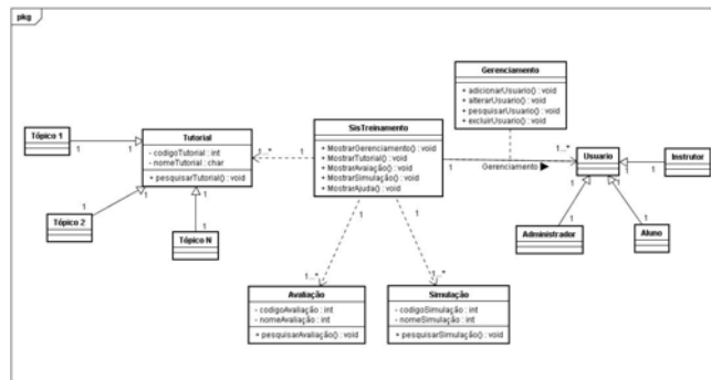
Fig. 9 Class diagram
