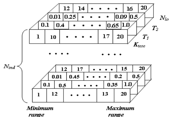
Fig. 4 Calculation of the entire population
