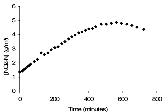
Fig. 20 Change in [NO_2-N] over time for initial load 8.00g NH_4-N/m^3 in ATS developed under HSL 1.96 m^3/m^2/d
