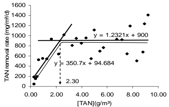
Fig. 9 Change in r TAN for initial load 8.00gNH 4 -N/m 3 in ATS developed under HSL 0.66 m 3 /m 2 /d
