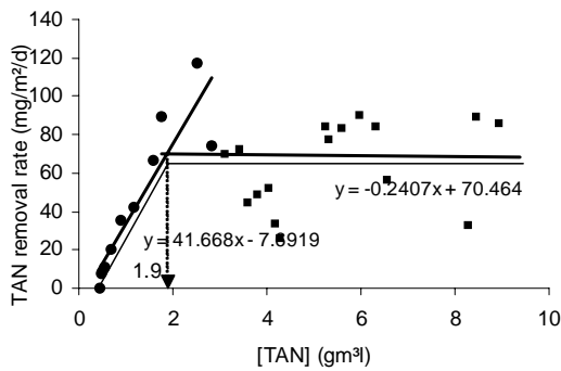
Fig. 11 Change in TAN for initial load 8.00gNH 4 -N/m 3 in ATS developed under HSL 1.96 m 3 /m 2 /d
