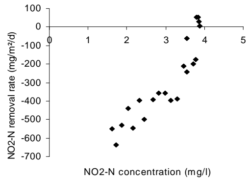
Fig. 15 Change in net NO 2 -N removal rate for initial load 3.11g NH 4 -N/m 3 in ATS developed under HSL 2.08 m 3 /m 2 /d
