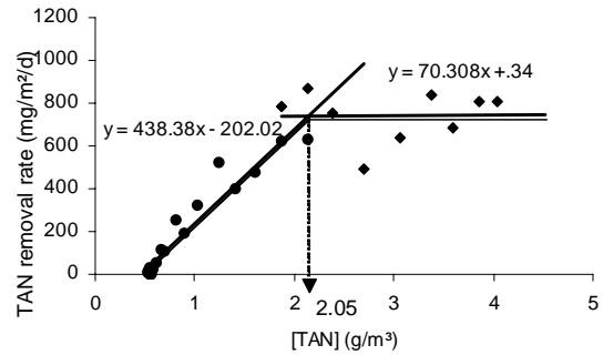
Fig. 7 Change in r TAN for initial load 5.13g NH 4 -N/m 3 in ATS developed under HSL 2.17 m 3 /m 2 /d
