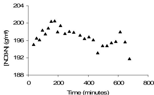
Fig. 22 Change in [NO 3 -N] over time for initial load 3.11g NH 4 -N/m 3 in ATS developed under HSL 0.62 m 3 /m 2 /d
