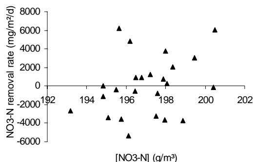
Fig. 23 Change in net NO 3 -N removal rate for initial load 3.11g NH 4 -N/m 3 in ATS developed under HSL 0.62 m 3 /m 2 /d
