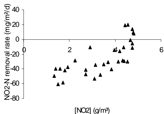
Fig. 21 Change in net NO 2 -N removal rate for initial load 8.00g NH 4 -N/m 3 in ATS developed under HSL 1.96 m 3 /m 2 /d
