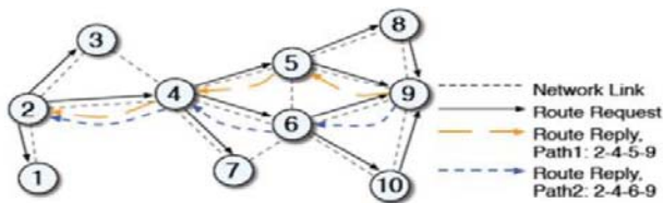
Fig. 2 DSR routing protocol[7]
