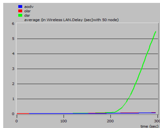
Fig.6 delay for 50 nodes
