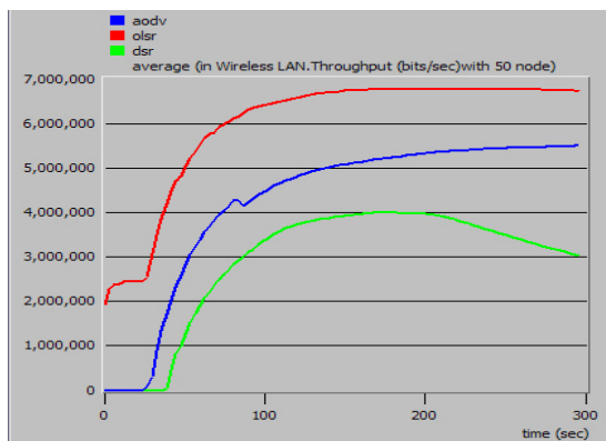
Fig. 4 throughput for 50 nodes
