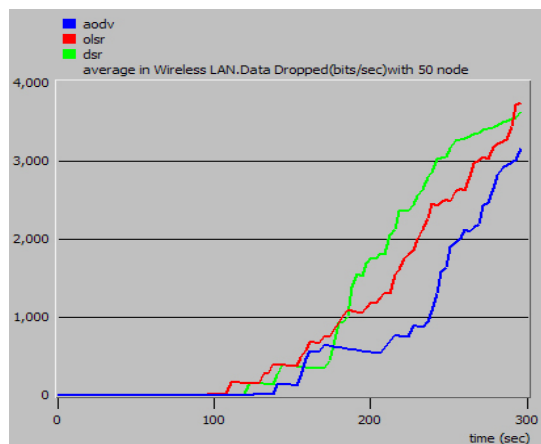
Fig. 8. packet drop rate for 50 nodes
