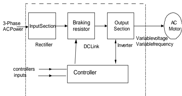
Fig. 1 Block diagram of conventional ASDs'
