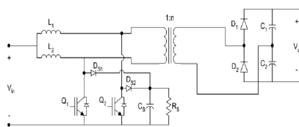
Fig. 4 Isolated boost converter topology
