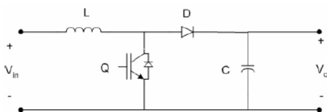
Fig. 3 Boost converter topology
