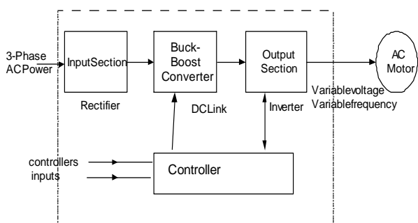
Fig. 2 Block diagram of ASD with isolated buck-boost converter
