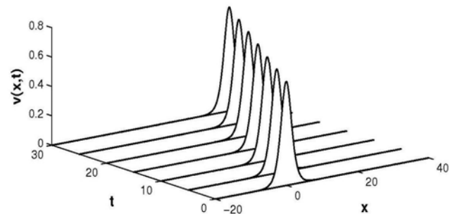
Fig. 1. The exact solutions of the amplitude u(x, t) and v(x, t) , versus the coordinate x, t of example. 3.1 with \lambda = 1 , and \alpha = 1 .
