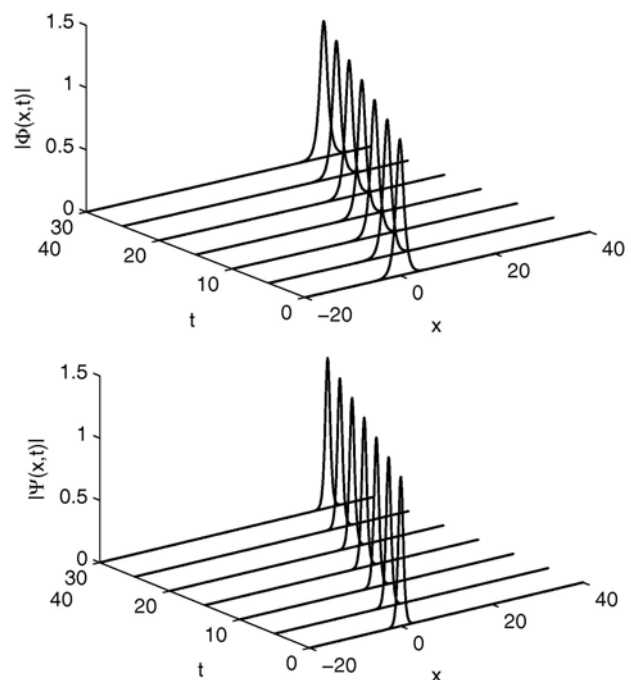
Fig. 2. The modulus of the amplitude |\Phi| and |\Psi| , versus the coordinate x, t of example. 3.3 with \nu = 1 , \alpha = 1 , \eta = \frac{1}{2} , and e = \frac{2}{3} .
