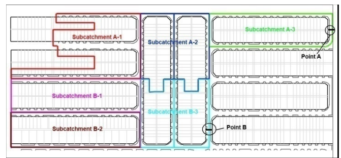
Fig. 2 Sampling/Outlet locations
