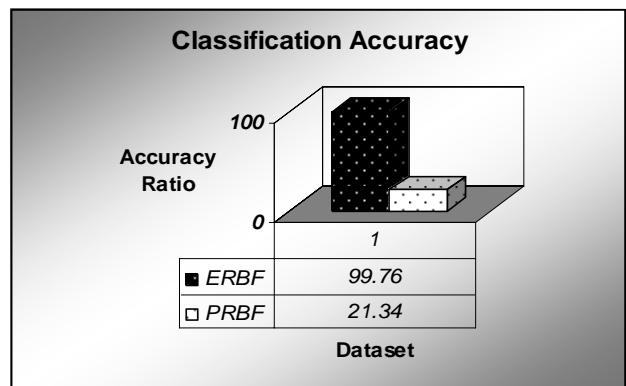
Fig. 2 Classification Accuracy
