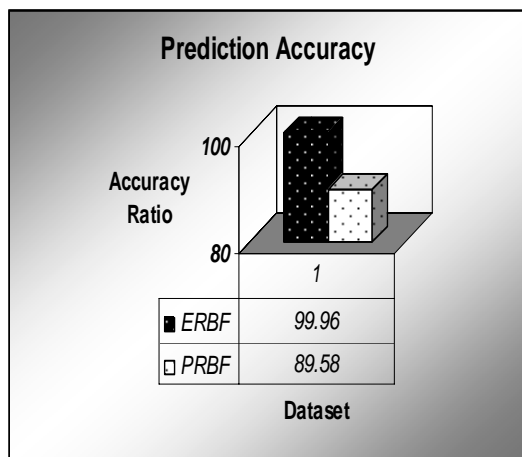
Fig. 3 Prediction Accuracy
