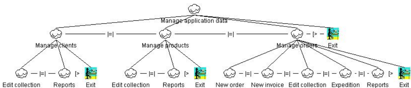
Fig. 1 Mapping of application functions onto user tasks
