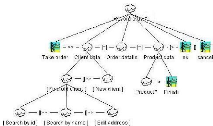
Fig. 3 Decomposition for the task "Record order"
