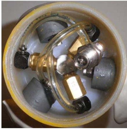
Fig. 5 Floatation system
