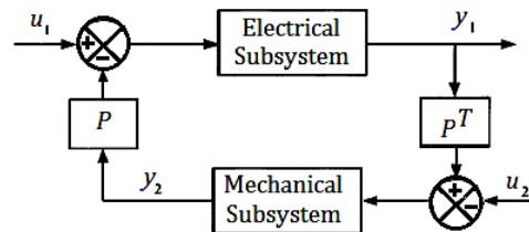
Fig. 1 Negative feedback interconnection of subsystems
