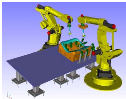
Fig. 7 Robot cell layout after applying cell configuration principle
