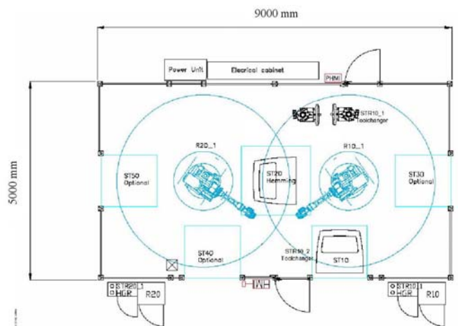
Fig. 6 Robot cell layout and operability region
