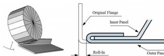
Fig. 1 Roller hemming process
