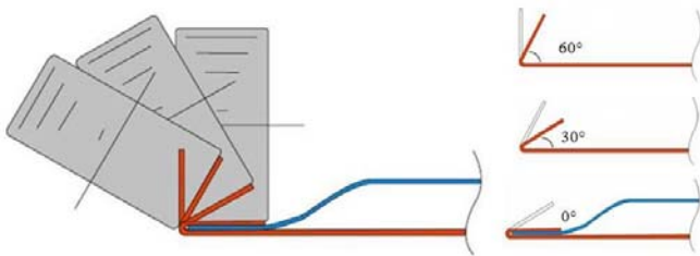
Fig. 2 Three steps in the roller hemming process
