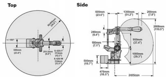
Fig. 5 Robot specifications and operability region
