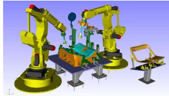
Fig. 3 Robot cell layout at Saab Automobile AB
