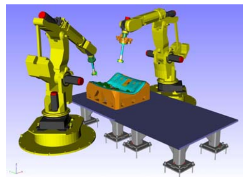
Fig. 4 Robot cell layout after applying task separation and robot coordination principles
