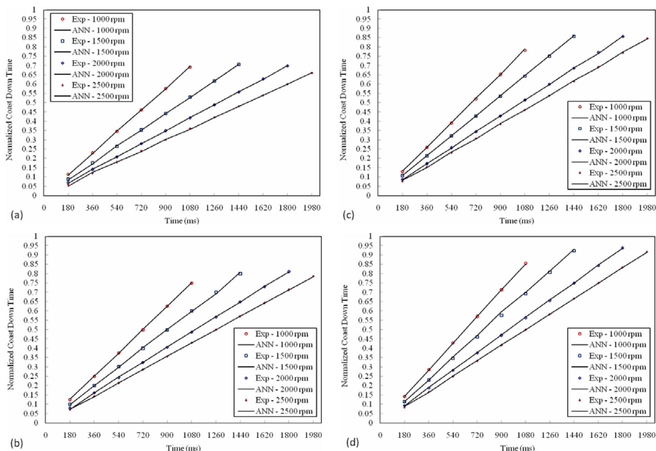
Fig. 9 Experimental and Artificial Neural Networks predicted CDT data for a) balanced, b) 22 gram-mm, c) 27 gram-mm and d) 32 gram-mm unbalance weights added at blower shaft speed of 1000 rpm, 1500 rpm, 2000 rpm and 2500 rpm
