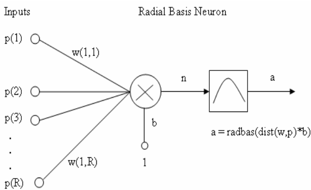
Fig. 5 Radial Basis Neuron Model
