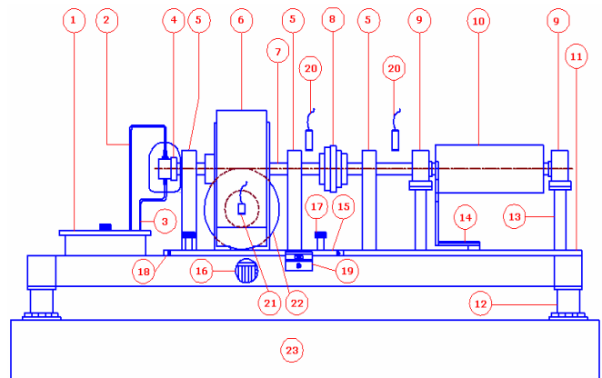
Fig. 1 Centrifugal Blower Experimental Test Rig
