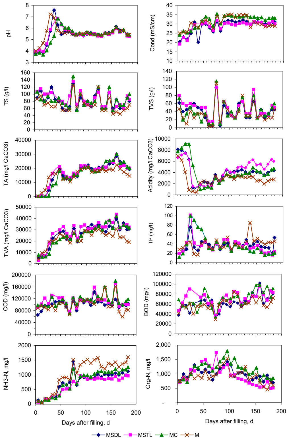
Fig. 4 Leachate characteristic variation over time
