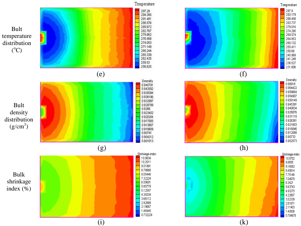
Fig. 5 Bulk distribution inside cavity with melt compressibility effect -- (a,c,e,g,i) without surface roughness, i.e. \delta_{upper}=\delta_{bottom}=0\mu\text{m} at both the upper and bottom halves and (b,d,f,h,k) with surface roughness, i.e. \delta_{bottom}=40\mu\text{m} at the bottom half and \delta_{upper}=0\mu\text{m} at the upper half
