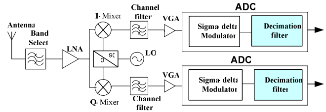
Fig. 1 Direct conversion homodyne receiver architecture
