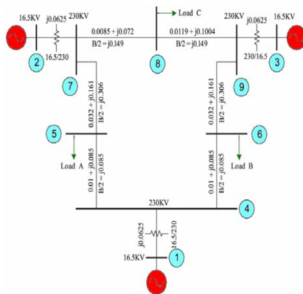
Fig. 1 The 3 machine 9 bus test case
