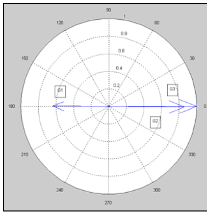
Fig. 4 Swinging at 100% increase in base generation of machine 3
