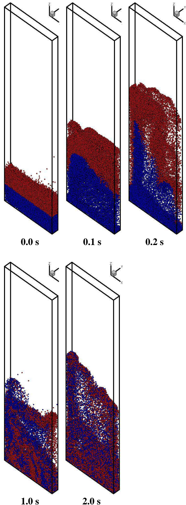
Fig. 1 Mixing behavior of dry particles in a gas fluidized bed. The fluidization velocity applied was 1.6 m s -1
