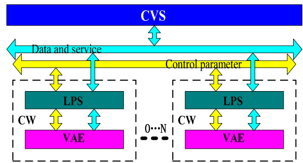
Fig. 3 Triple hierarchy distributed collaborative visualization framework
