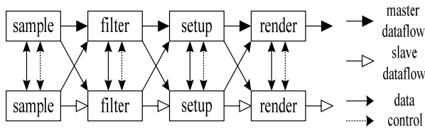
Fig. 2 Pipeline in collaboration mode
