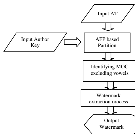
Fig. 2 Watermark extraction process
