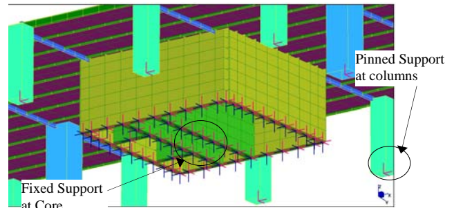
Fig. 8 Strand7 3D view showing support conditions
