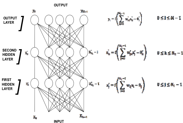
Fig. 1 Standard Multi layer perceptron architecture
