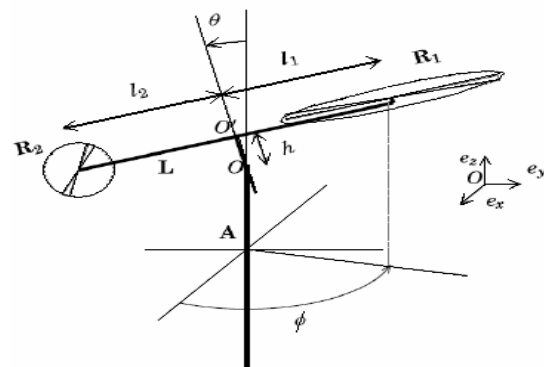
Fig. 1 Helicopter process configuration
