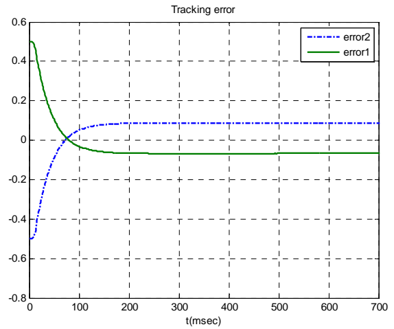
Fig. 6 Tracking error (unknown parameter control law)
