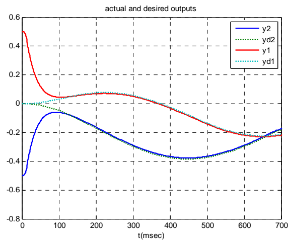
Fig. 7 Actual and desired outputs (adaptive feedback linearization)
